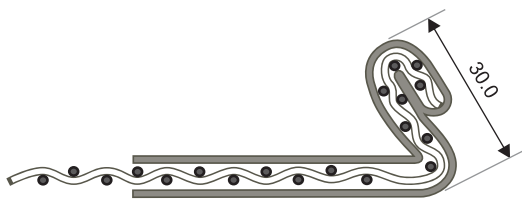
Sheet metal hook with double fold ( less than 2mm thickness )
