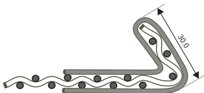
Sheet metal hook ( for 2mm to 7mm thickness )
